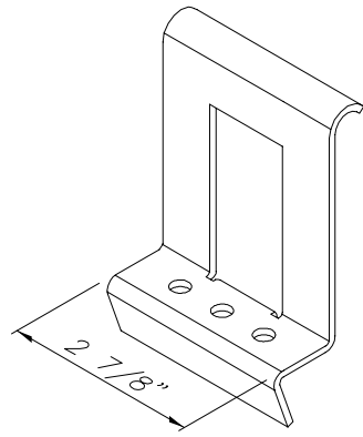
A-25 ATTACHMENT CLIP FOR 4" VERSAPANEL PANEL 12 GAGE ASTM-653 GRADE 50, G90 GALV.
