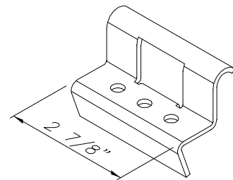
A-19 ATTACHMENT CLIP FOR 1 3/4" VERSAPANEL PANEL 12 GAGE ASTM-653 GRADE 50, G90 GALV.
