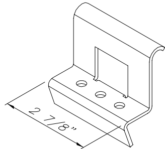
A-24 ATTACHMENT CLIP FOR 2.50" VERSAPANEL PANEL 12 GAGE ASTM-653 GRADE 50, G90 GALV.
